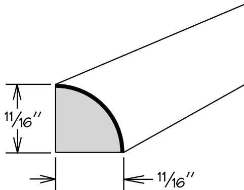
QUARTER ROUND
