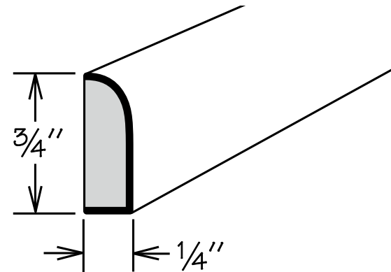
SCRIBE
